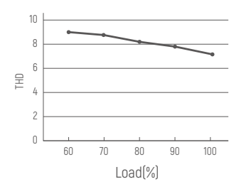
THD vs Load
