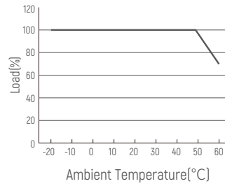
Derating Curve
