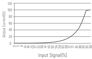
Dimming Curve
